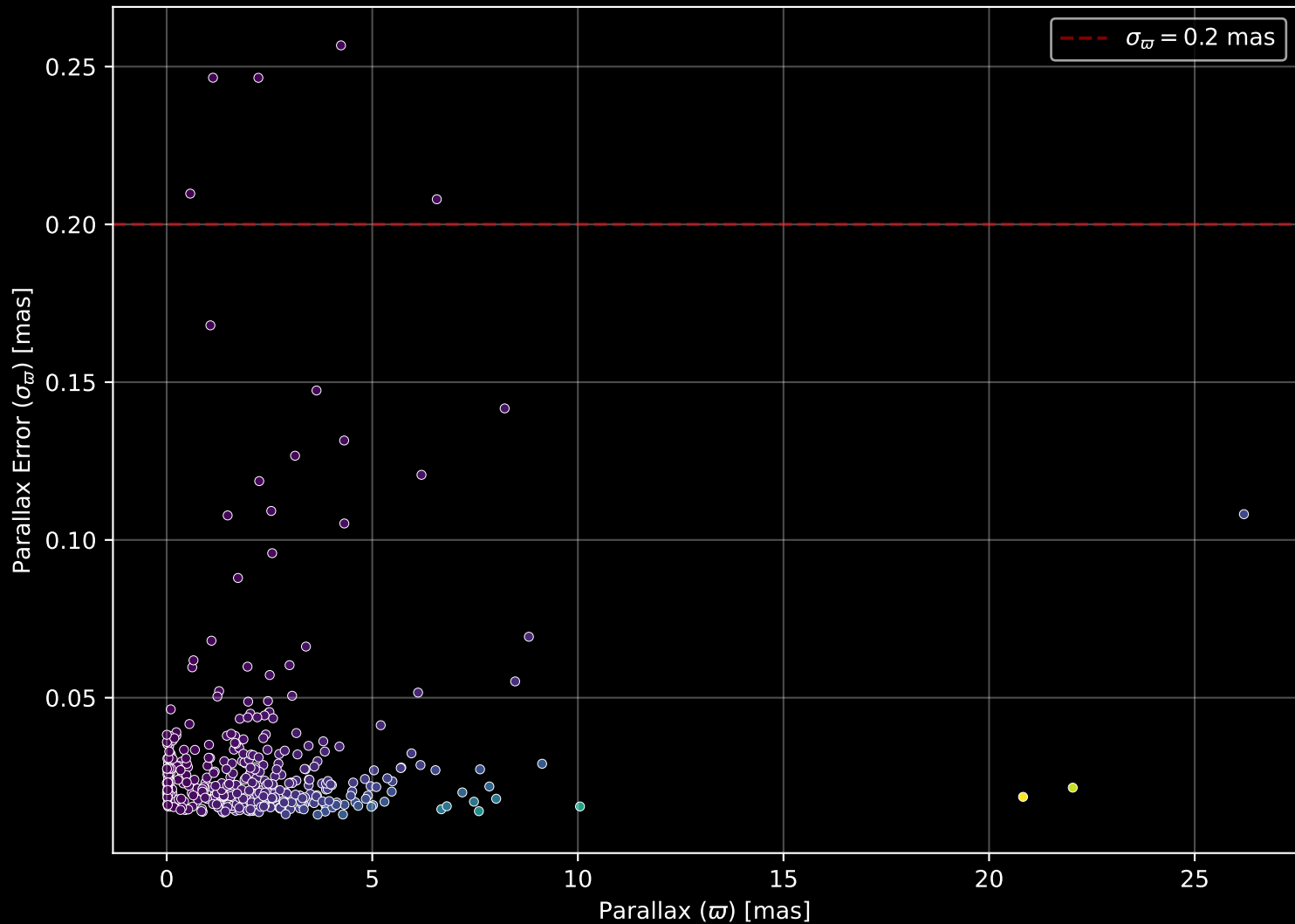
APOGEE DR17 Field: [M53] Parallax Quality (n= 407)
