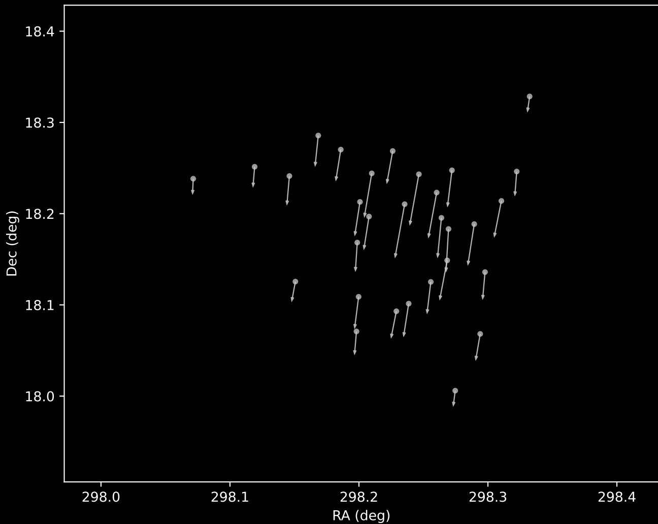
APOGEE DR17 Cluster 15 Proper Motion Vectors (n=30)
