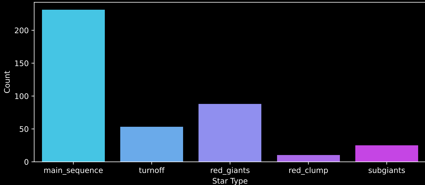
APOGEE DR17 Field: [M53] Count plot of Star Type
