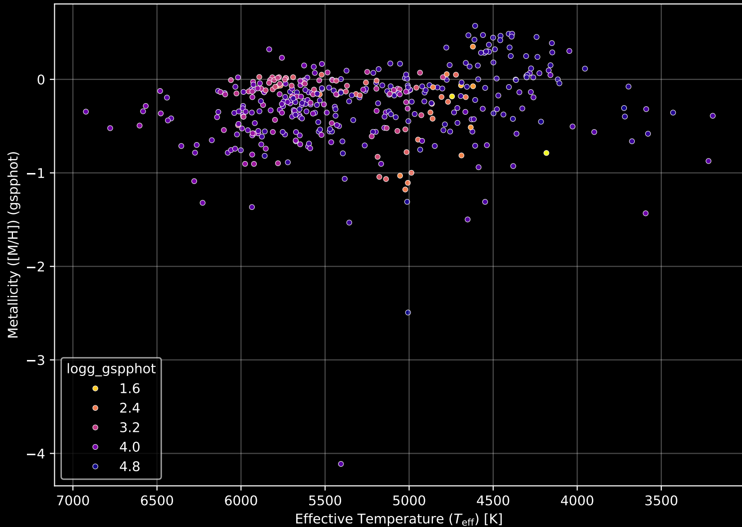
APOGEE DR17 Field: [M53] Stellar Population Parameters (n= 407)
