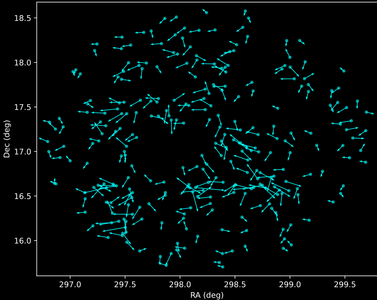
APOGEE DR17 Noise Stream Proper Motion Vectors (n=280)
