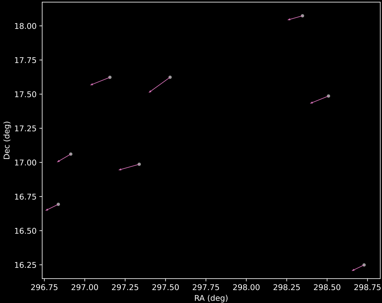
APOGEE DR17 Cluster 12 Proper Motion Vectors (n=8)
