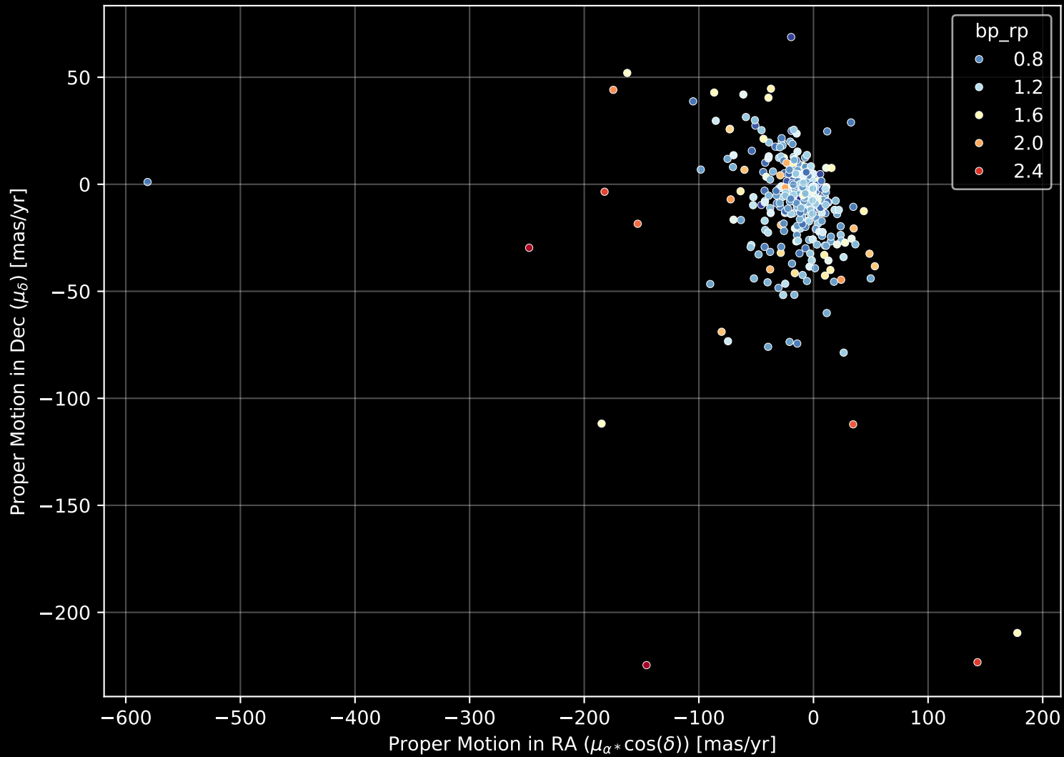
APOGEE DR17 Field: [M53] Proper Motion Diagram (n= 407)
