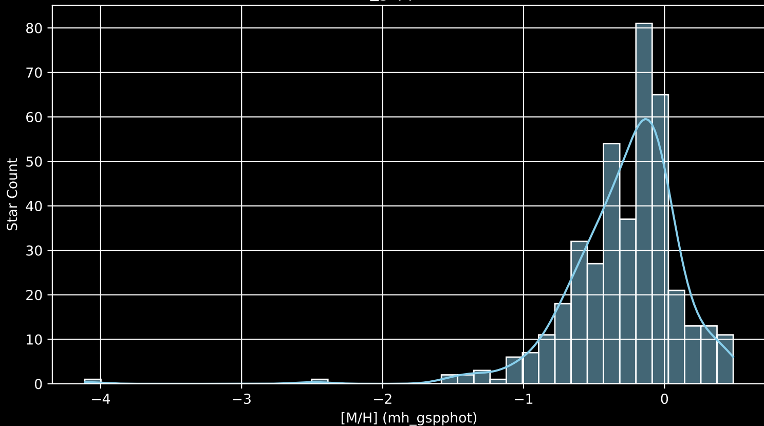
APOGEE DR17 Field: [M53 [M/H] (mh_gspphot) (n= 406)
