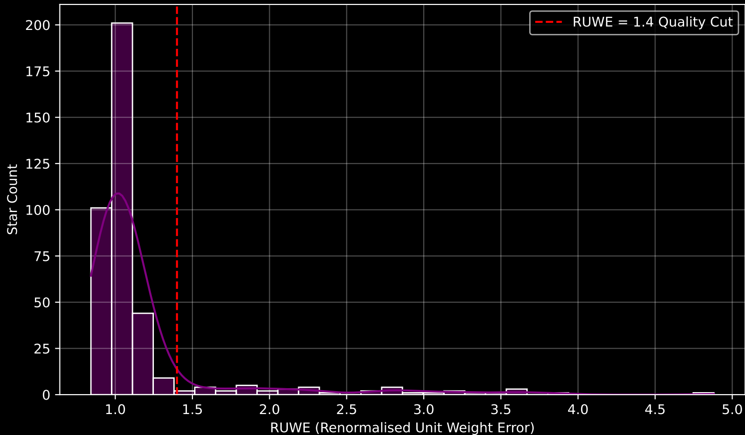
GAPOGEE DR17 Field [M53] RUWE Distribution (n= 395)
